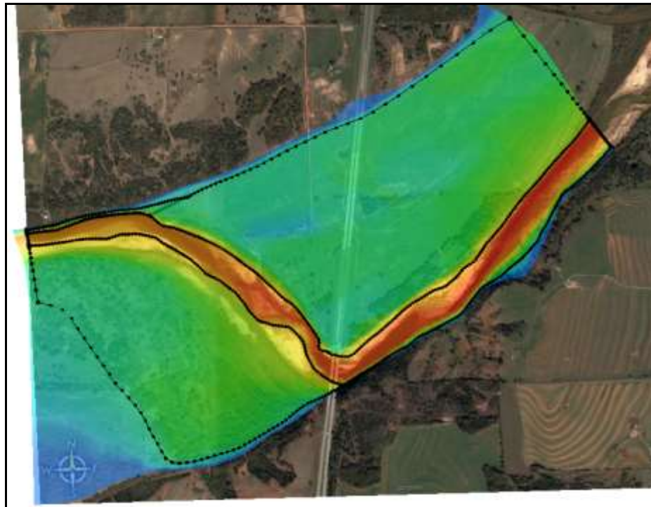
Figure 1 Conceptual model extents with a background image
